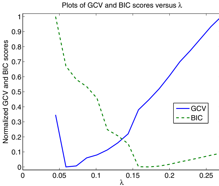
Figure 1. Tuning parameters and their corresponding BIC and GCV scores for the Framingham data. The scores are normalized to the range [0, 1].
